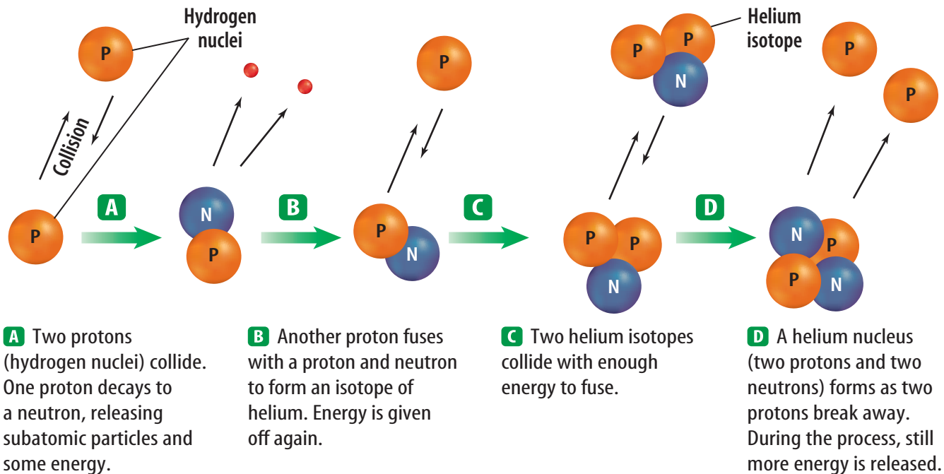
Figure 12 Fusion of hydrogen into helium occurs in a star's core. Infer what happens to the "lost" mass during this process.
